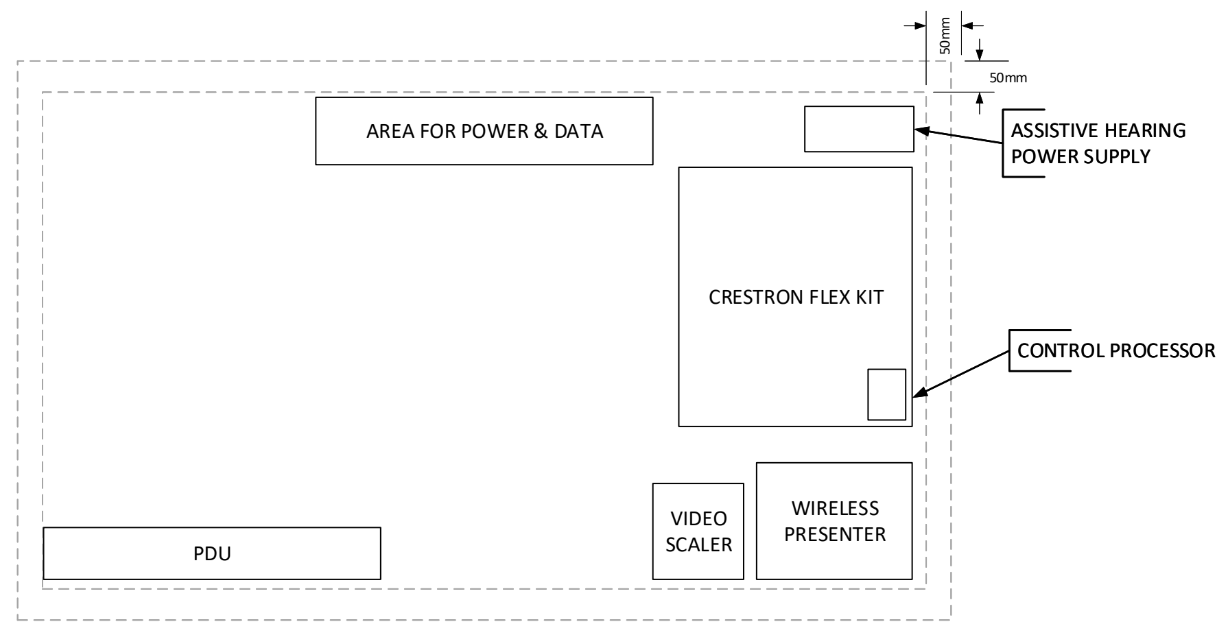
2 MEDIUM MEETING/COLLABORATION SYSTEM – EQUIPMENT LAYOUT BEHIND LCD SCREEN - NTS
