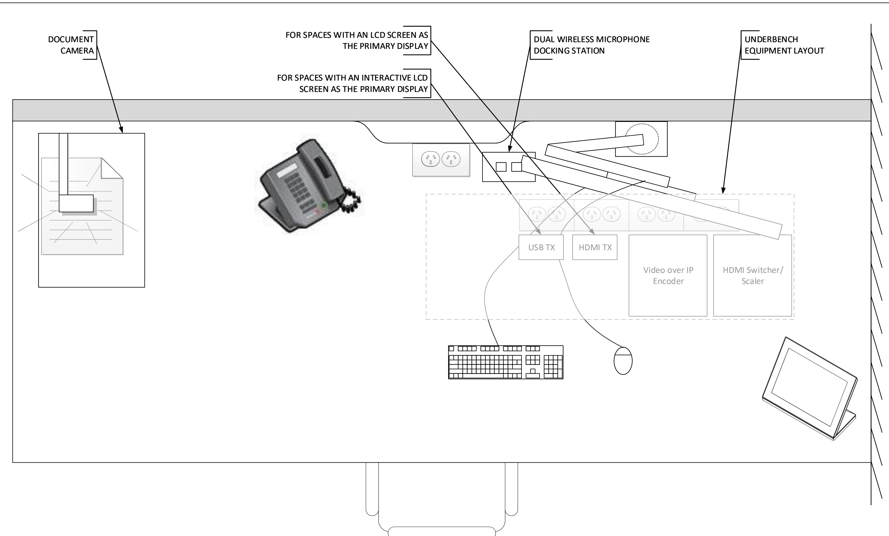
2 PLAN – ACADEMIC'S DESK (RIGHT) NTS
