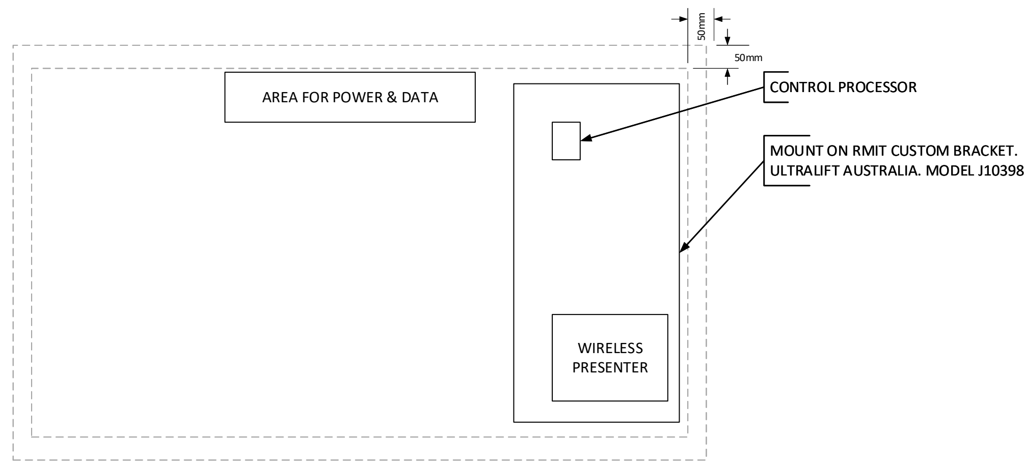
1 SMALL MEETING/COLLABORATION SYSTEM – EQUIPMENT LAYOUT BEHIND LCD SCREEN - NTS
