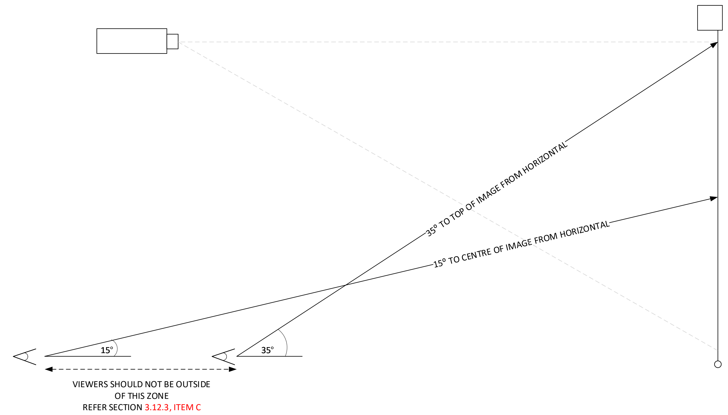
2 - VIEWING SITELINES - VERTICAL NTS
