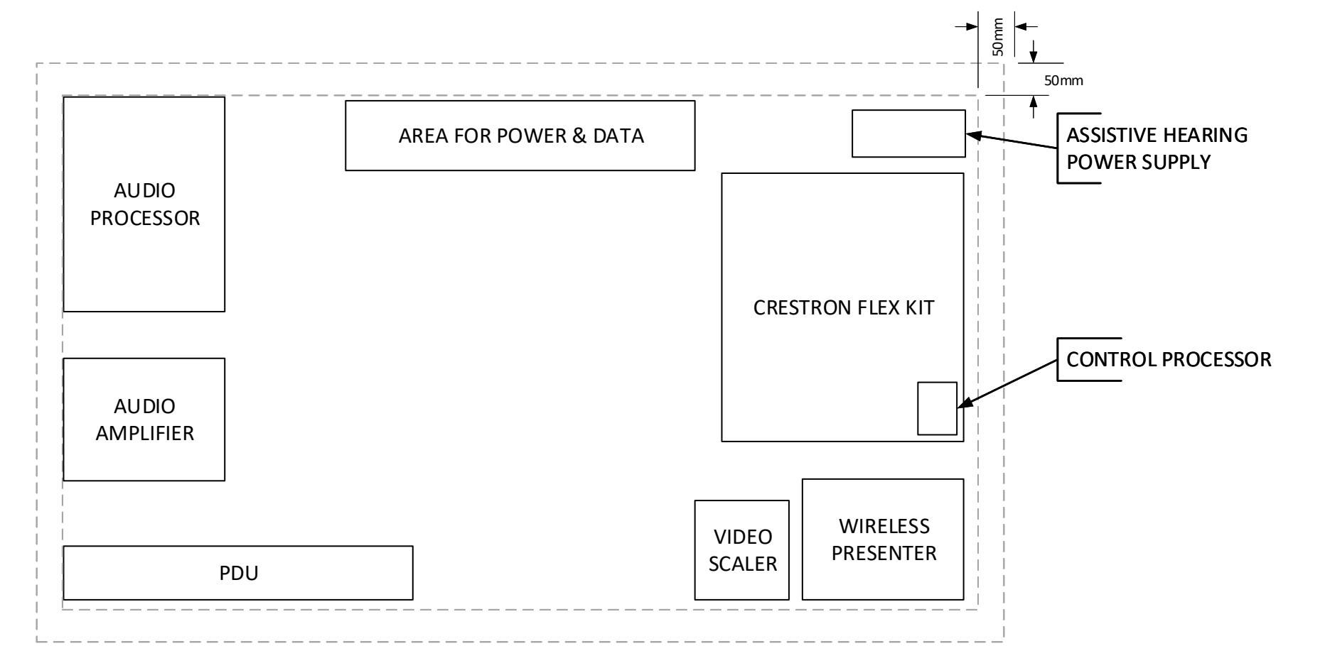
3 LARGE MEETING/COLLABORATION SYSTEM – EQUIPMENT LAYOUT BEHIND LCD SCREEN - NTS
