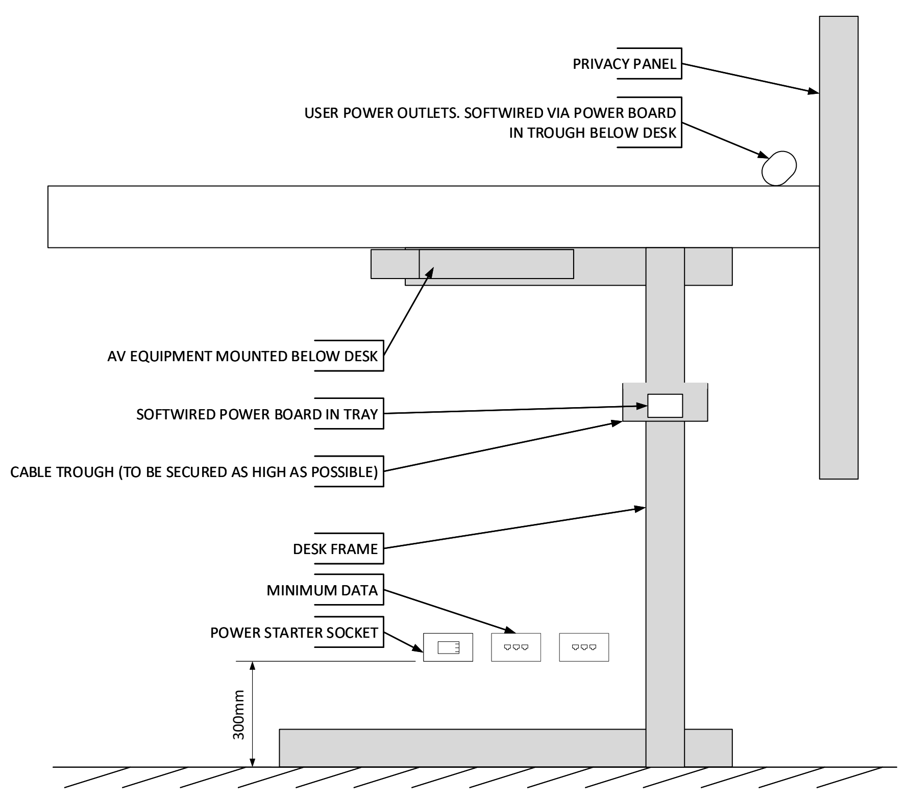
3 SECTION – ACADEMIC'S DESK NTS
