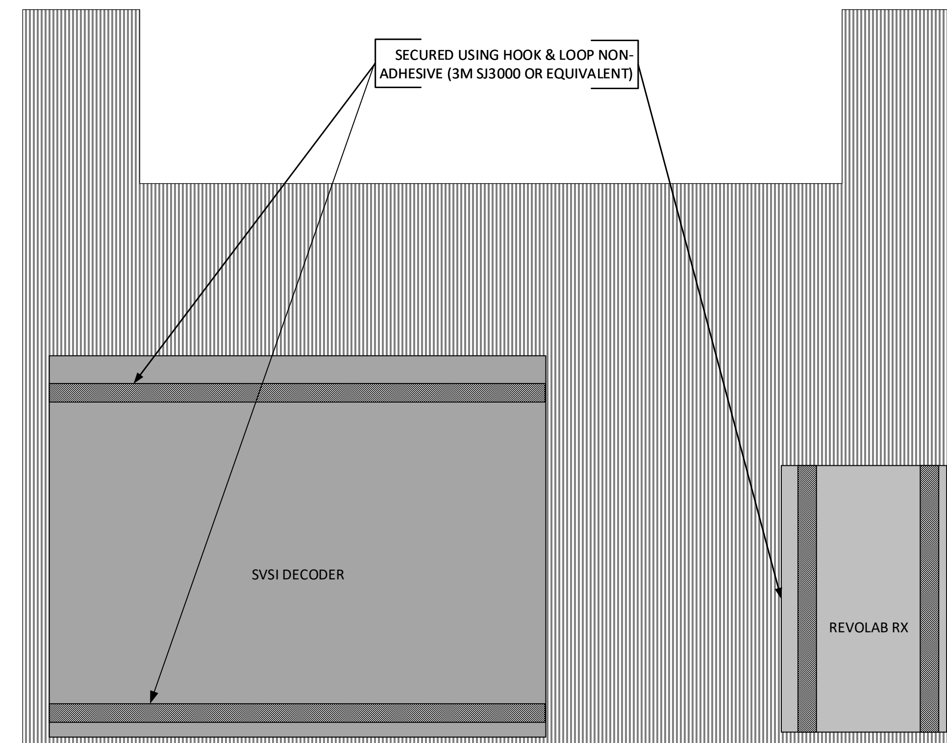
2 PLAN VIEW OF SLOTTED SHELF - NTS
