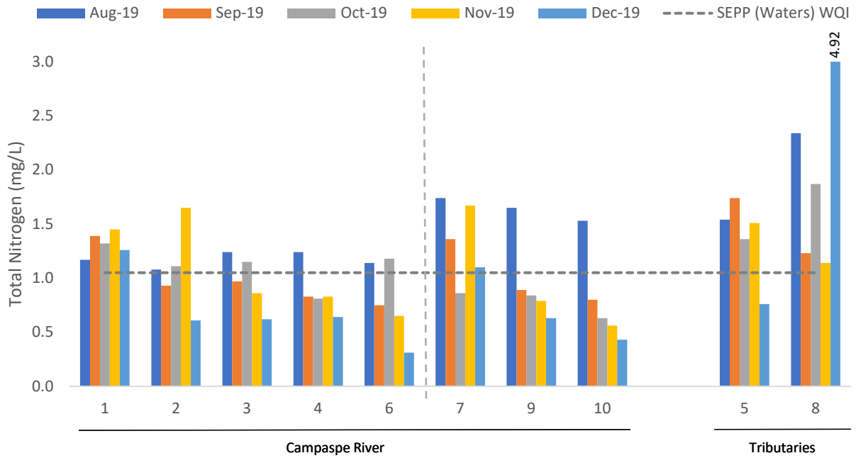
Figure 8. Monthly total nitrogen concentrations in surface waters during Year 2 monitoring from August to December 2019. The vertical dashed line indicates Kyneton WRP discharge point between Sites 6 and 7. Where concentrations were below the limit of reporting these have been presented as zero.
