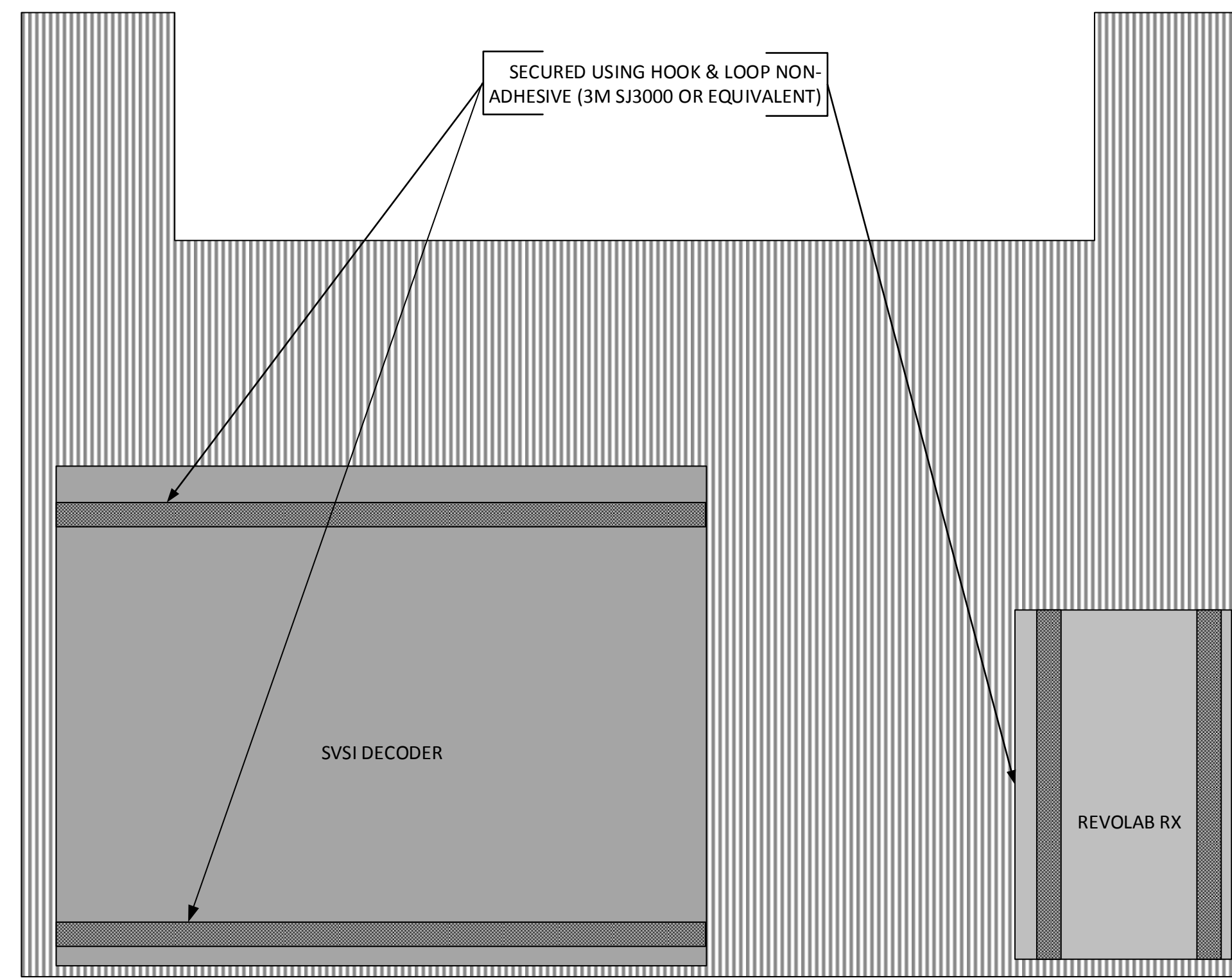
2 PLAN VIEW OF SLOTTED SHELF - NTS
