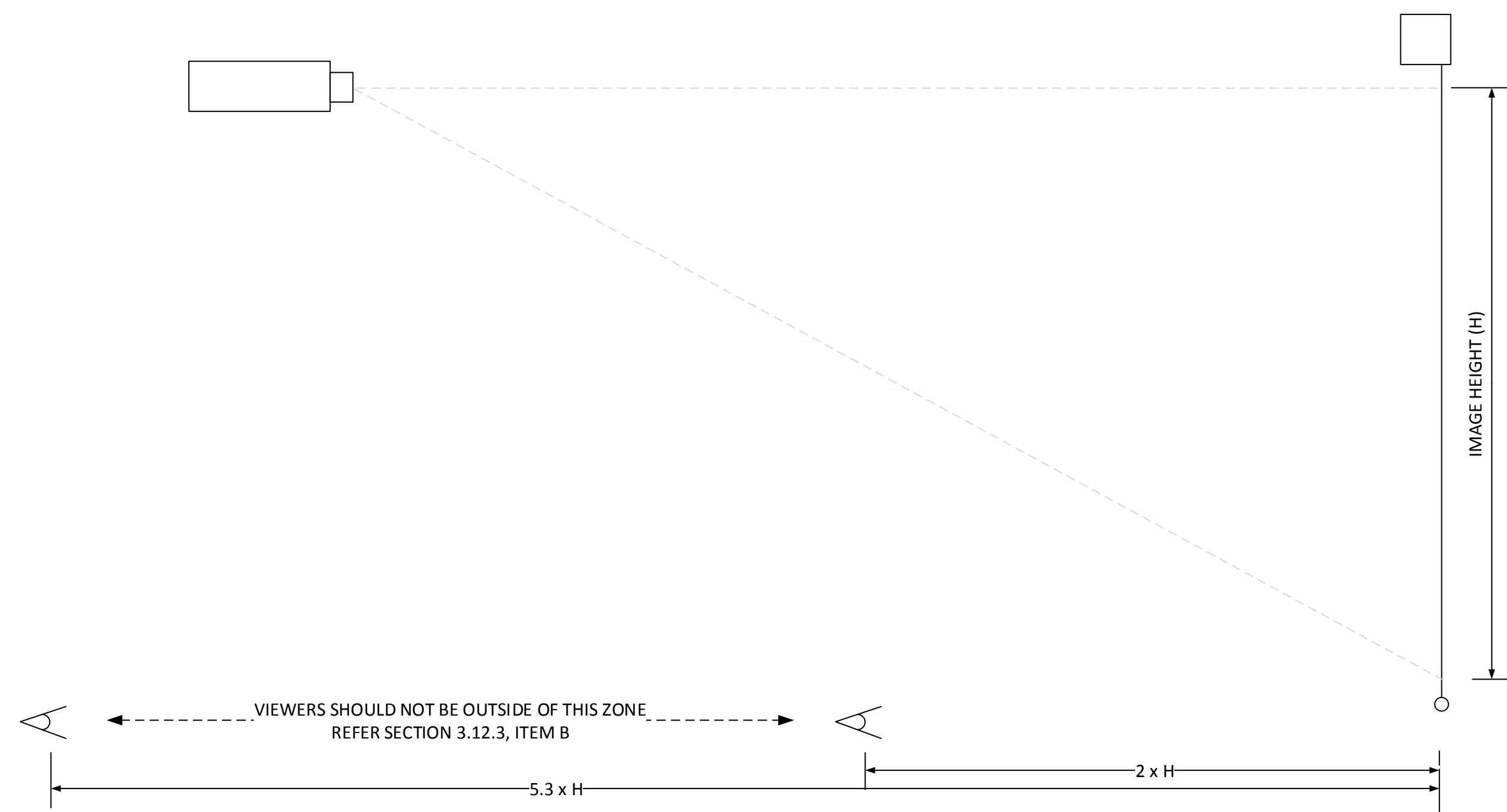
3 - VIEWING DISTANCES AGAINST IMAGE SIZE (720P) NTS
